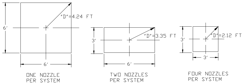
FIGURE 4-2 INDIVIDUAL NOZZLE COVERAGE
