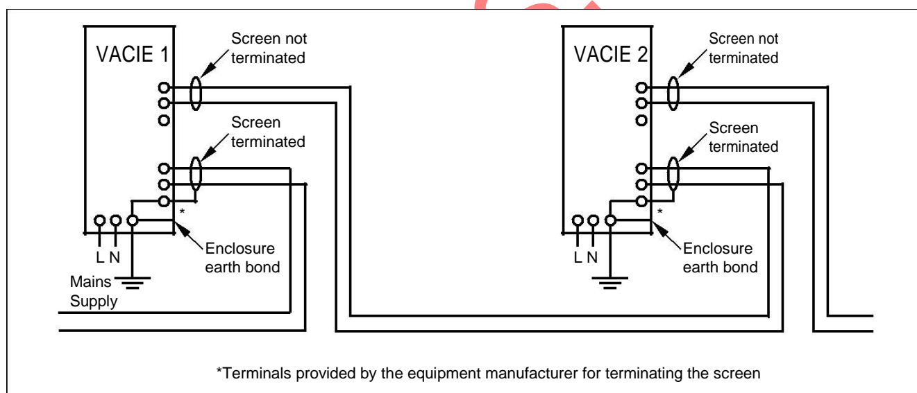
Figure 6 Example of network wiring
