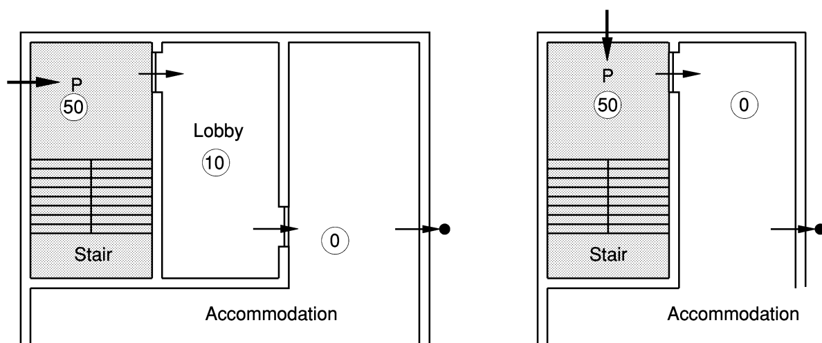
a) Pressurization to stairs only, with or without lobby
