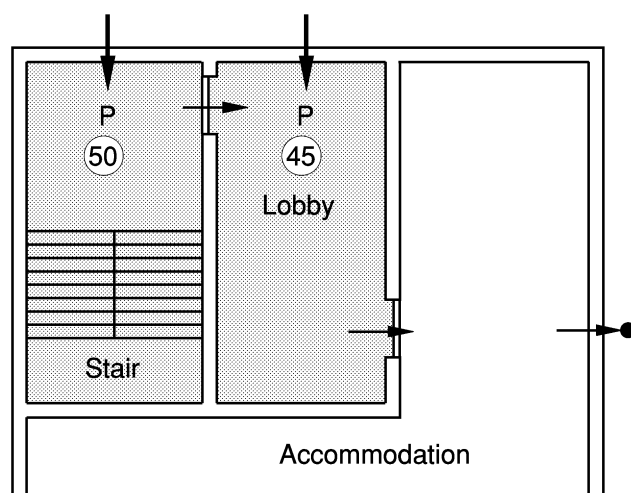
b) Pressurization to stairs and all associated lobbies
