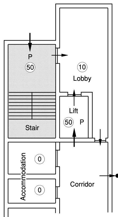
c) Pressurization to stairs and liftwell
