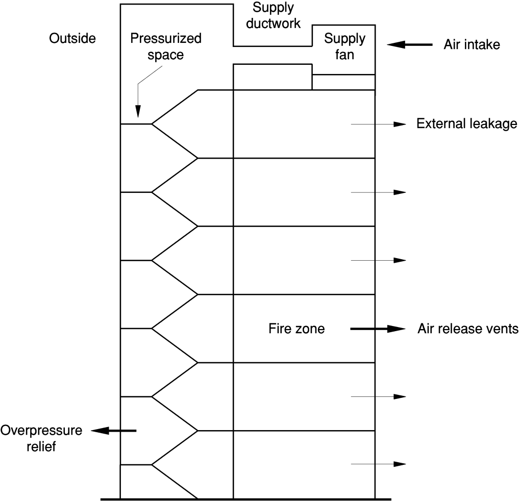
Figure 7a — Principles of a typical stair pressure differential system for means of escape (continued)
