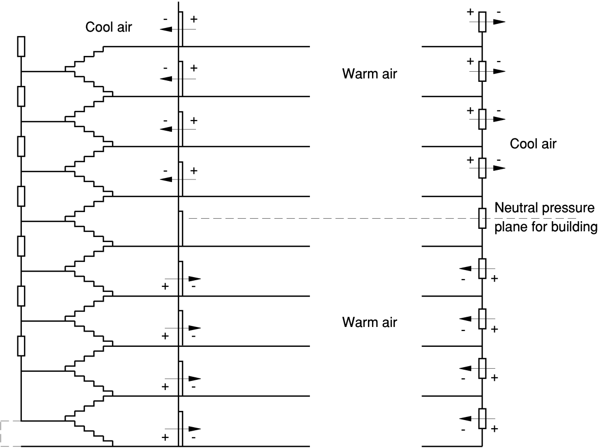
b) Stack effect in a heated building
