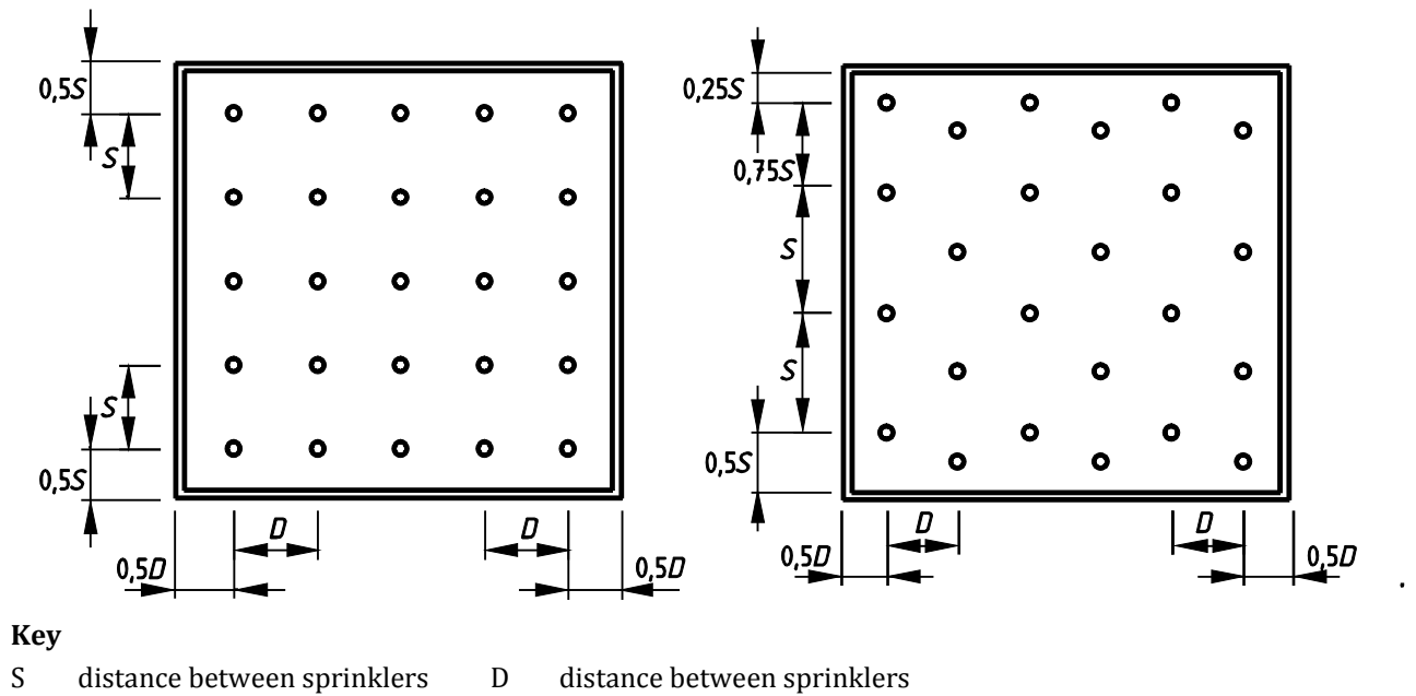
Figure 8 — Ceiling sprinkler spacing
