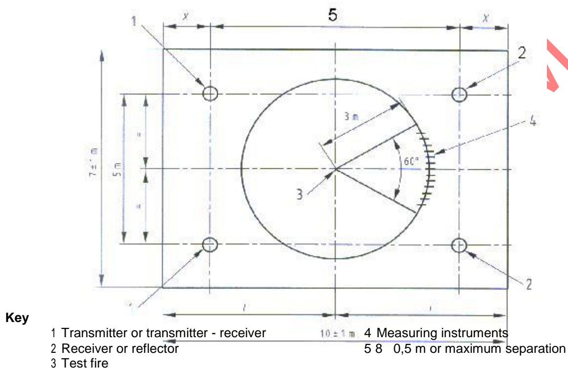
Figure B.1 - Plan view of detectors, position of fire and measuring instruments
