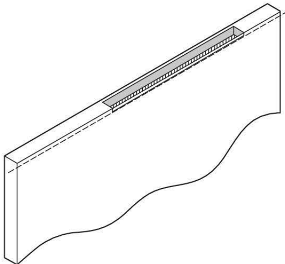
FIGURE A.6.7.1.2 Mortise Cutout in Top of Door Leaf for Overhead Door Stop. The dotted line represents the height of the door stop on the door frame.
