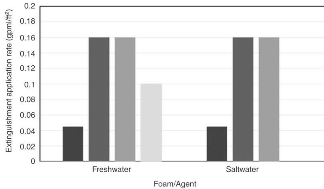
Application Rate
