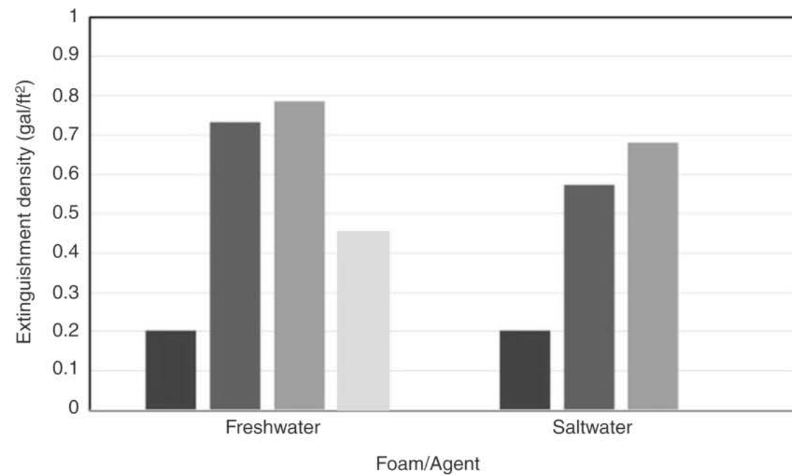
Extinguishment Density
