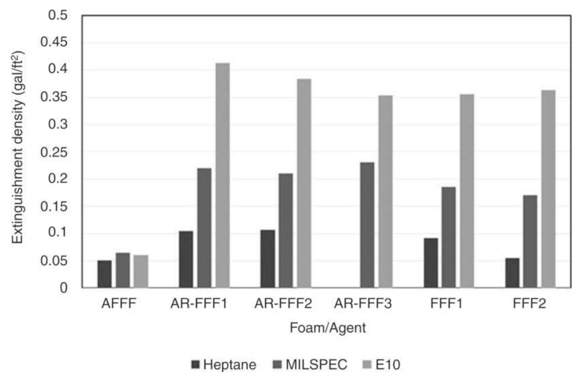
Extinguishment Density
