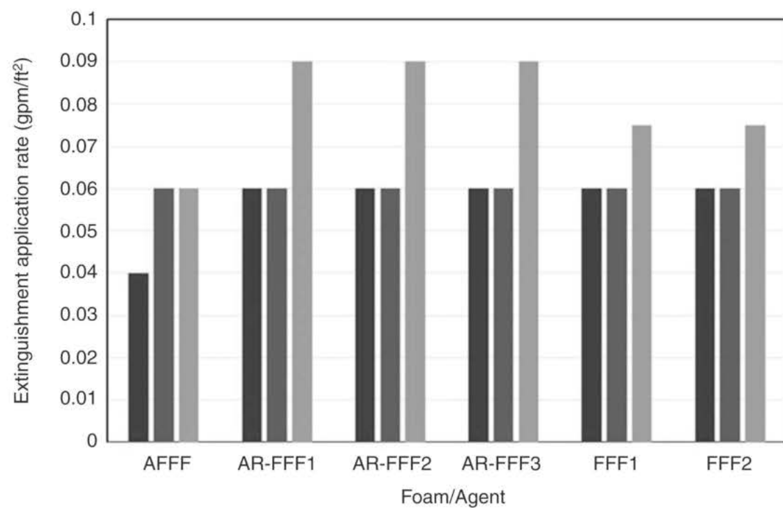
Application Rate
