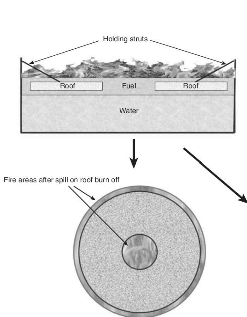
FIGURE I.1.2.4 Fire Areas During Roof Test.
