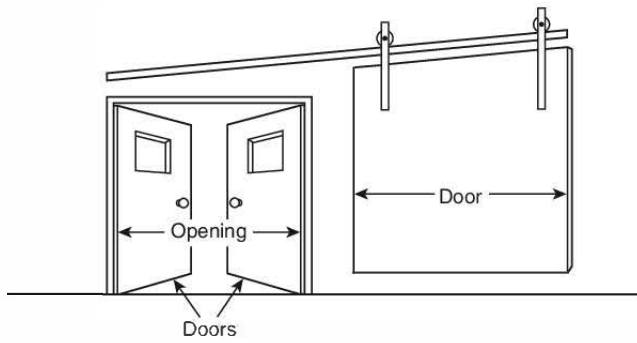
FIGURE A.5.8.3(a) Swinging Door and Sliding Door Configuration for Egress Purposes in an HC Fire Wall.
