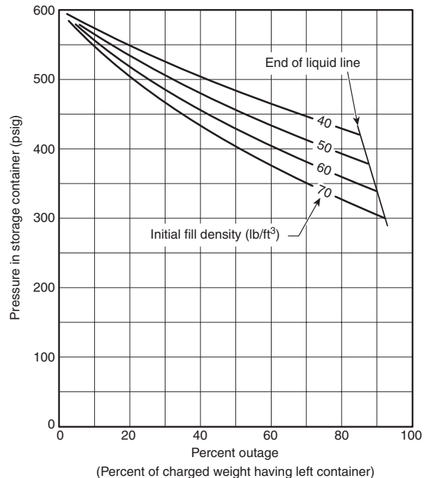
FIGURE H.1(b) Calculated Pressure Recession for 600 psig Storage.
